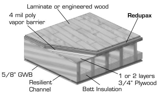
Typical Wood Construction
