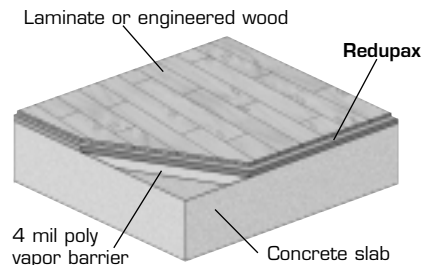
Typical Concrete Slab Construction
